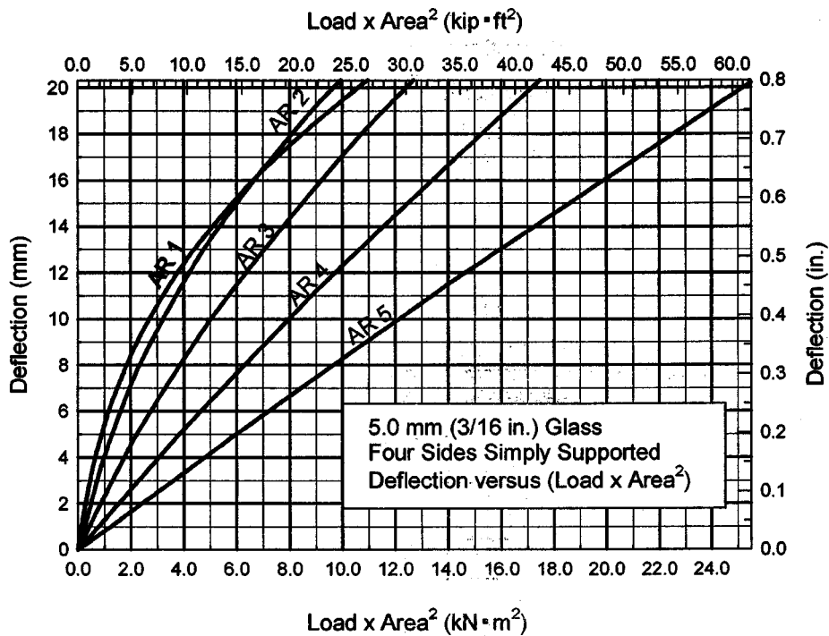
FIG. A1.5 (upper chart) Nonfactored Load Chart for 5.0 mm ( \frac{3}{16} in.) Glass with Four Sides Simply Supported (lower chart) Deflection Chart for 5.0 mm ( \frac{3}{16} in.) Glass with Four Sides Simply Supported
