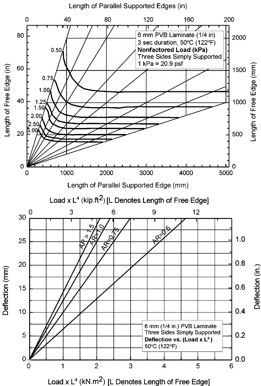
FIG. A1.35 (upper chart) Nonfactored Load Chart for 6.0 mm (¼ in.) Laminated Glass with Three Sides Simply Supported (lower chart) Deflection Chart for 6.0 mm (¼ in.) Laminated Glass with Three Sides Simply Supported
