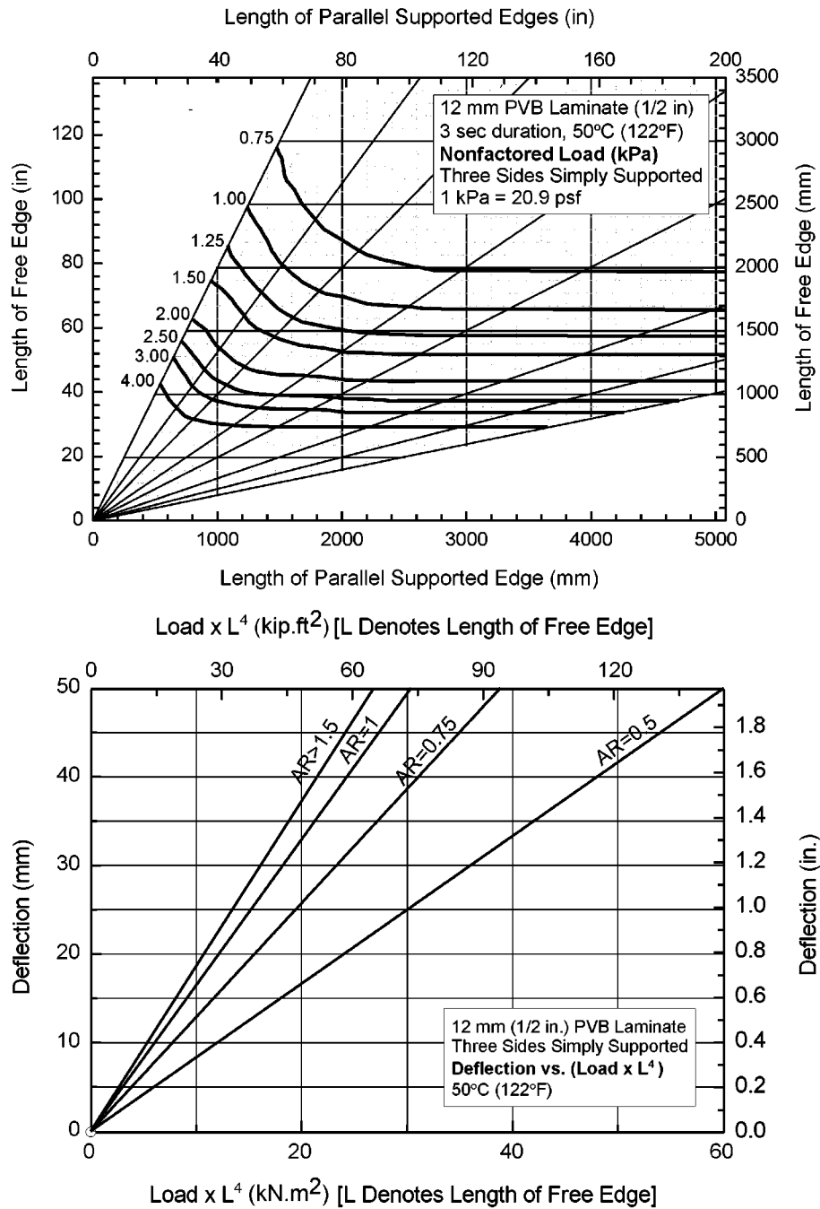
FIG. A1.38 (upper chart) Nonfactored Load Chart for 12.0 mm (½ in.) Laminated Glass with Three Sides Simply Supported (lower chart) Deflection Chart for 12.0 mm (½ in.) Laminated Glass with Three Sides Simply Supported
