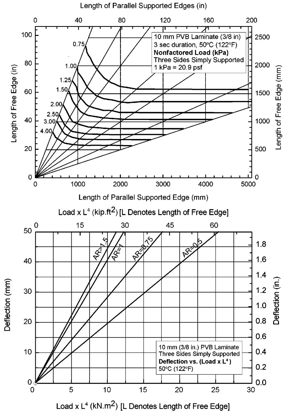
FIG. A1.37 (upper chart) Nonfactored Load Chart for 10.0 mm (3/8 in.) Laminated Glass with Three Sides Simply Supported (lower chart) Deflection Chart for 10.0 mm (3/8 in.) Laminated Glass with Three Sides Simply Supported
