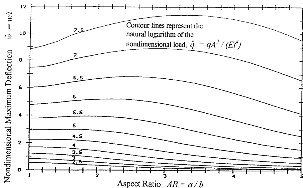
FIG. X1.1 Deflection Chart
