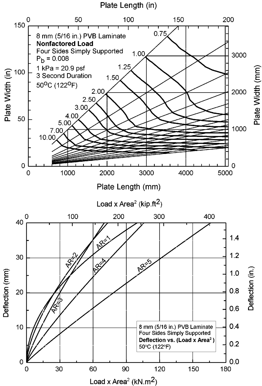
FIG. A1.29 (upper chart) Nonfactored Load Chart for 8.0 mm ( \frac{5}{16} in.) Laminated Glass with Four Sides Simply Supported (lower chart) Deflection Chart for 8.0 mm ( \frac{5}{16} in.) Laminated Glass with Four Sides Simply Supported
